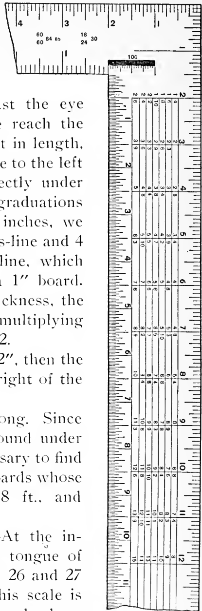
FIG. 27. BOARD MEASURE TABLE.
